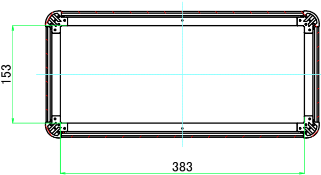
C-C (1:6)
